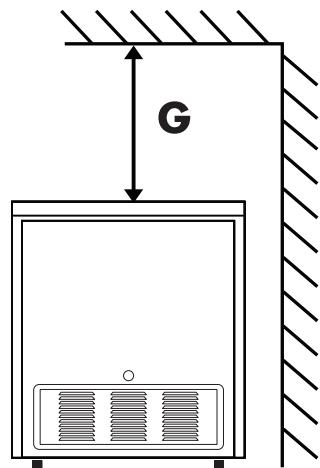
• Figure 3. Side view
